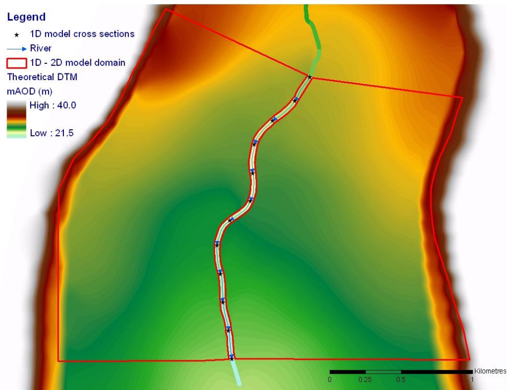
Figure 3-7 The Theoretical Model – model layout and topography
