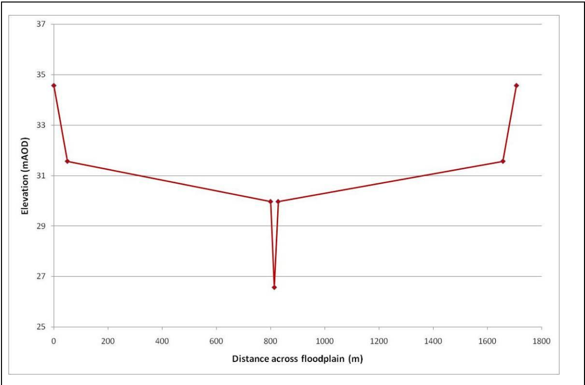
Figure 3-6 Theoretical model floodplain cross section
