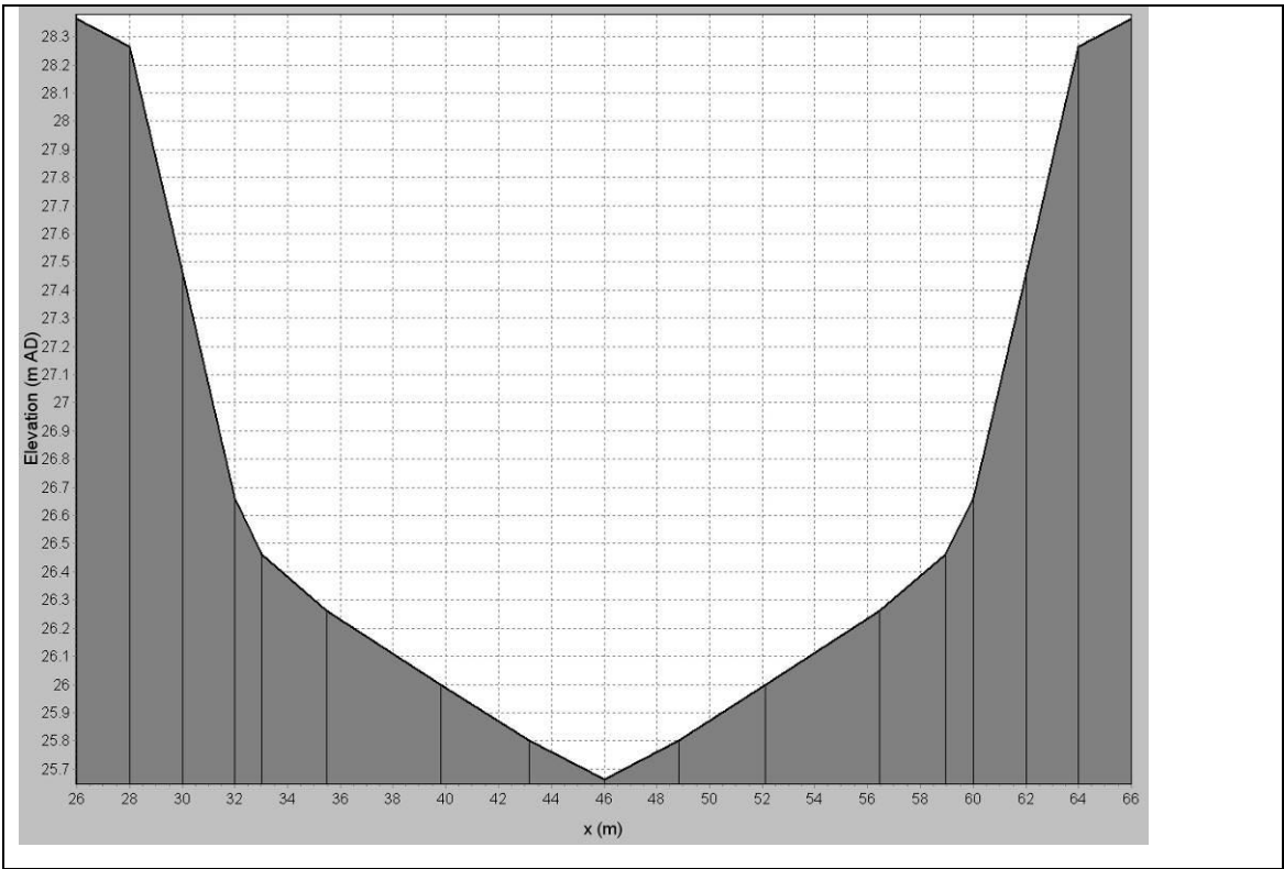
Figure 3-5 Theoretical model river cross section
