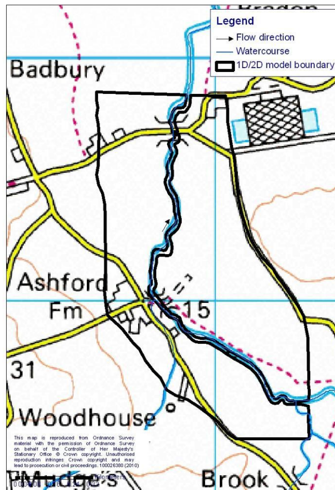
Figure 3-3 The Isle at Ashford Mill – site location
