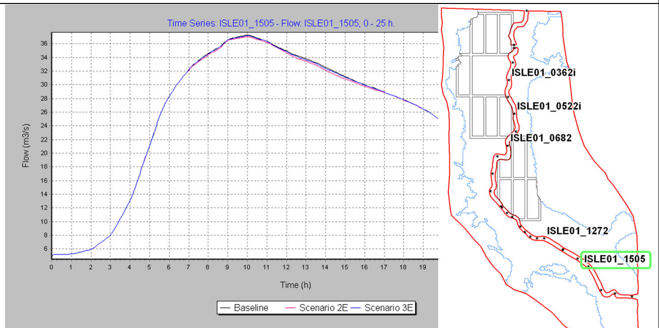
Figure 4-3 Isle at Ashford Mill – Main channel flood hydrographs (modelled floodplain in red, plantation layout in black and Flood Zone 3 extent in blue)
