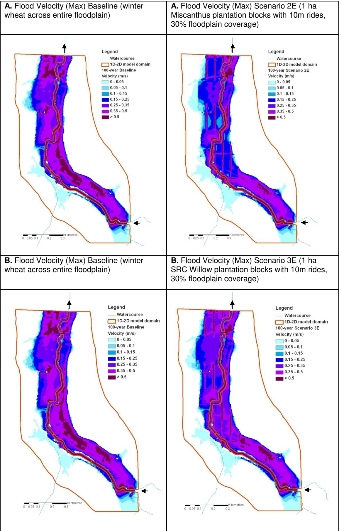
Figure 4-2 Isle at Ashford Mill – Flood velocity patterns
