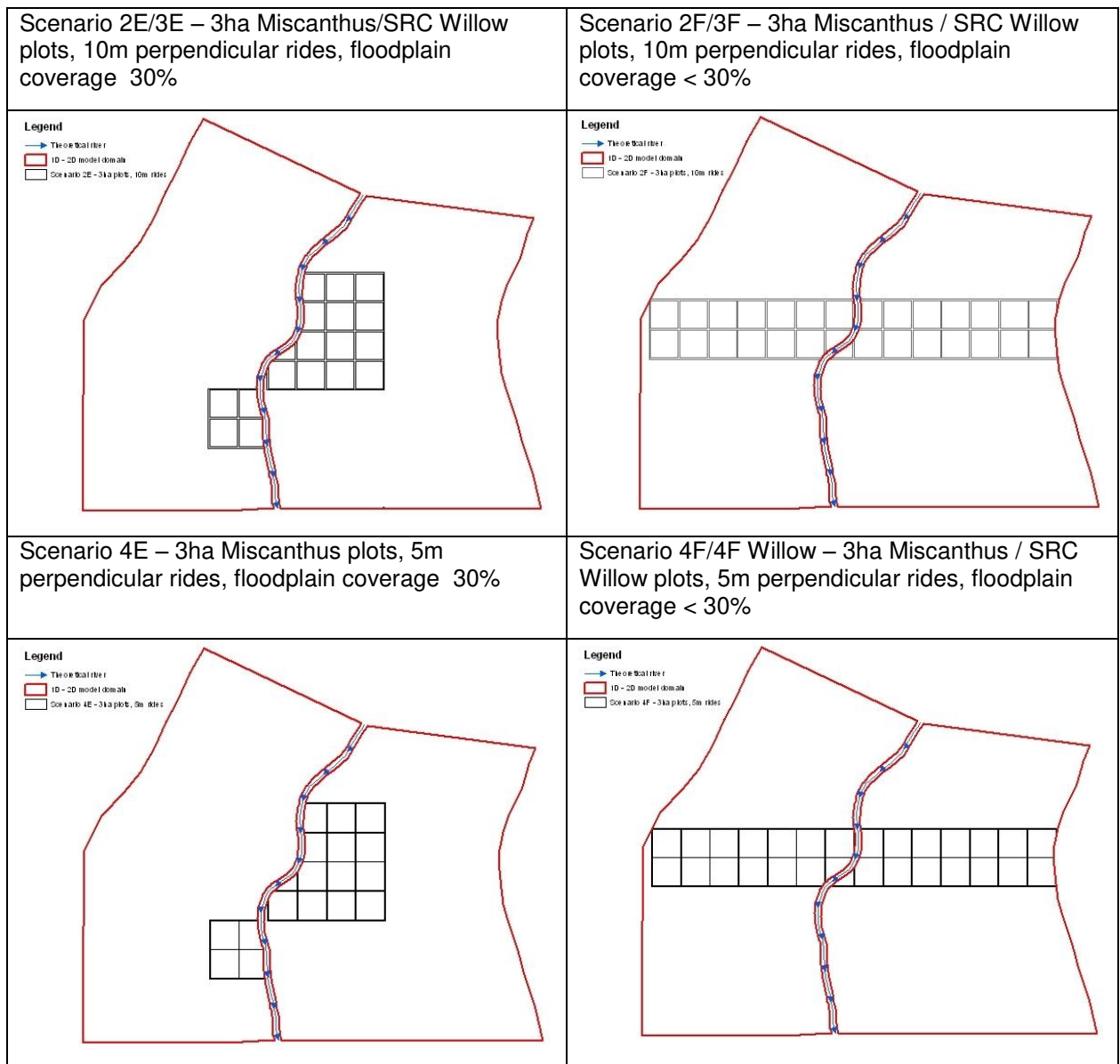
Figure 3-8 Modelled scenario configurations for Isle at Ashford Mill (the modelled floodplain area is shown in red, river in blue, plantation configuration with rides/headlands in black and the arrows signify the direction of river flow)
