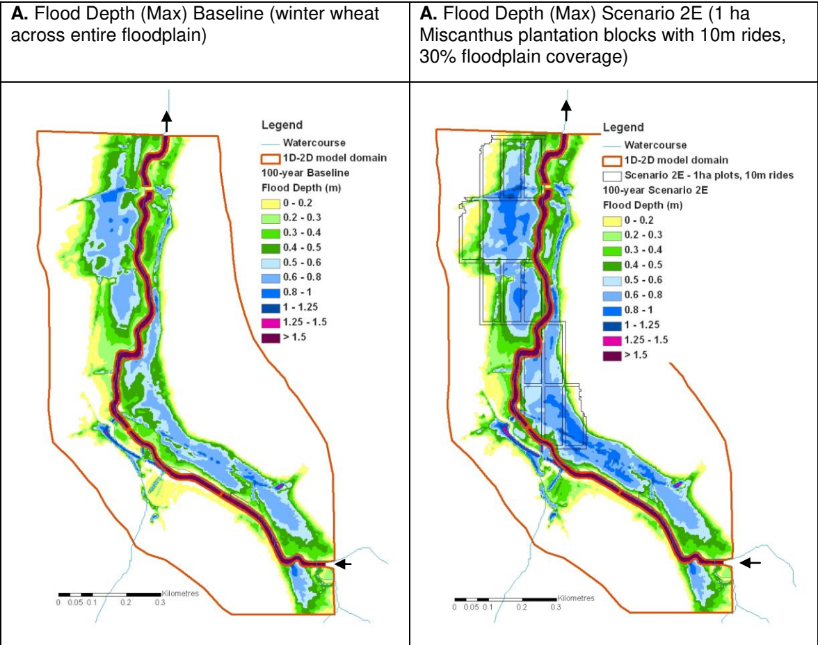
Figure 4-1 Isle at Ashford Mill – Flood depth patterns
