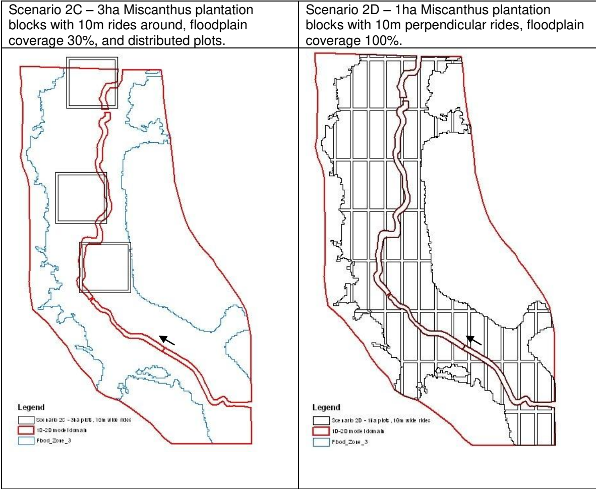
Figure 2-3 An example of modelling scenario layouts (2D model domain in red, extent of Flood Zone 3 in blue and plantation plots with rides around in black, arrow signifies the direction of flow)
