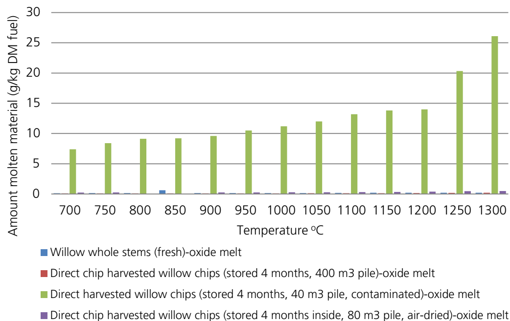
Figure 3. Estimated amount of oxide melt formed on combustion of fresh whole willow stems and of by sand/soil) or indoors. direct-chip harvested willow stored in a large stack (400 m 3), a small stack (40 m3, contaminated)
