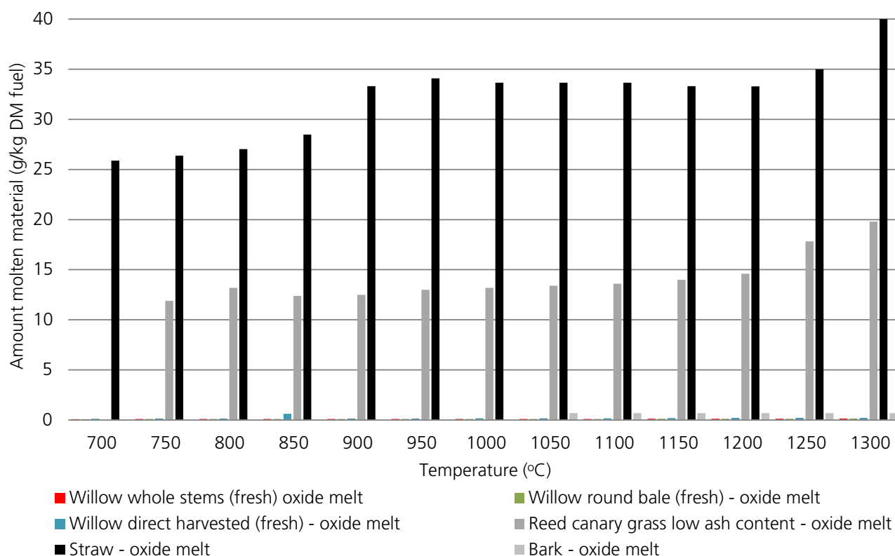
Figure 2. Estimated amount of oxide melt formed on combustion of three different fresh willow samples and of other typical biofuels.
